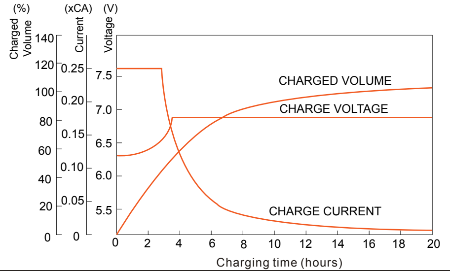
Constant voltage charging characteristic (0.25CA, 25°C)
