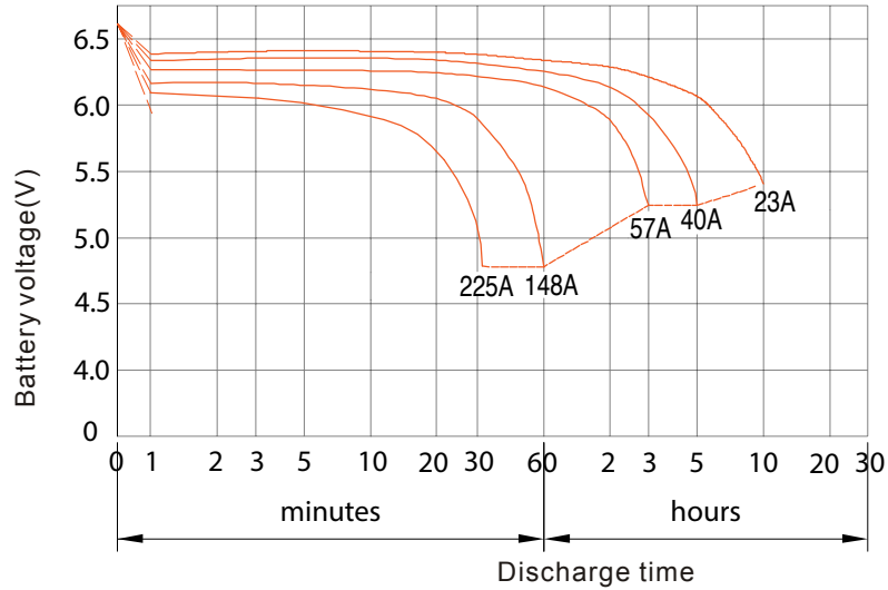
Discharge characteristic (25°C)
