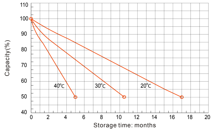
Self-discharge characteristic
