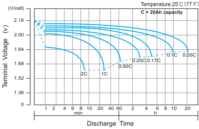
Discharge current characteristic (25°C)
