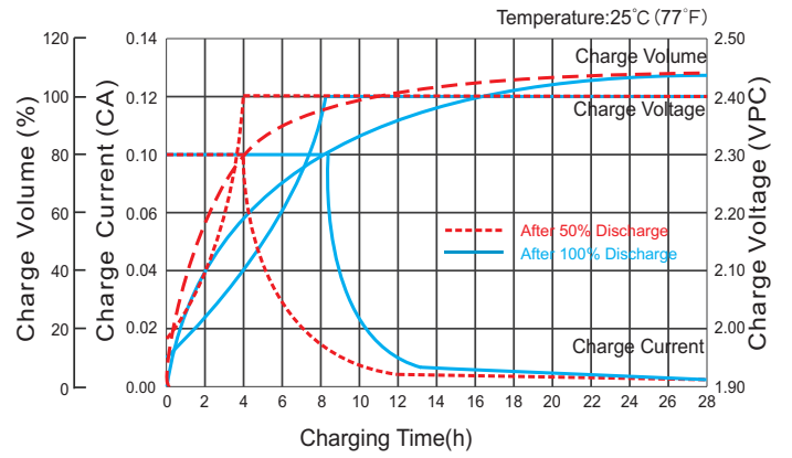
Constant voltage charging characteristic (0.25CA, 25°C)
