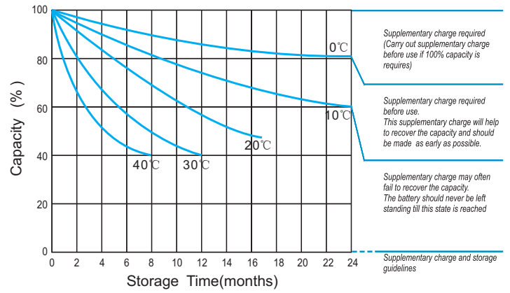
Self-discharge characteristic
