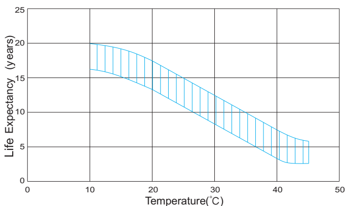
Temperature effects on float life
