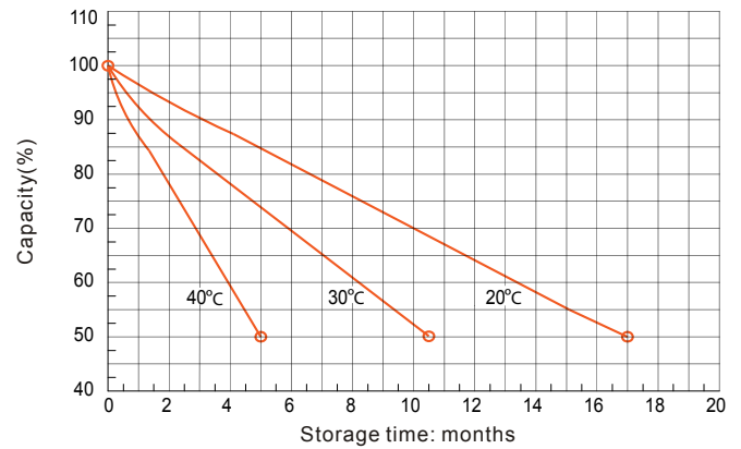
Self-discharge characteristic
