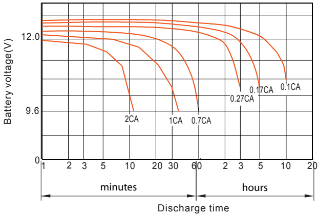
Discharge characteristic (25°C) Current displayed as multiples of CA
