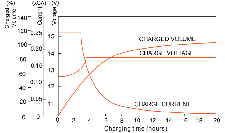
Constant voltage charging characteristic (0.25CA, 25°C)
